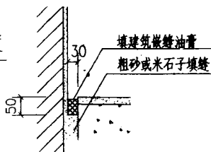
(C) 变形缝
