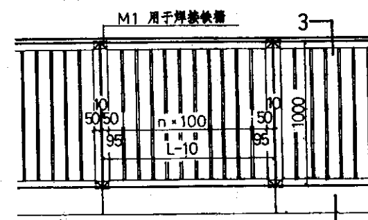
③ 窗井铁箍
