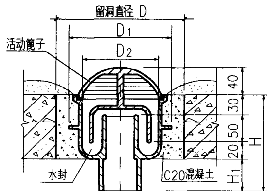
II型地漏
