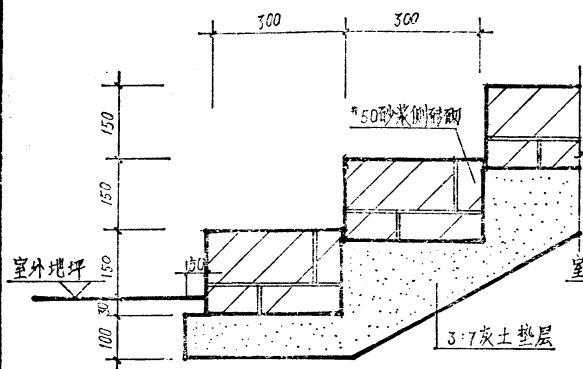
① 砖砌台阶
