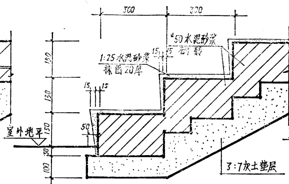
② 砖砌台阶
