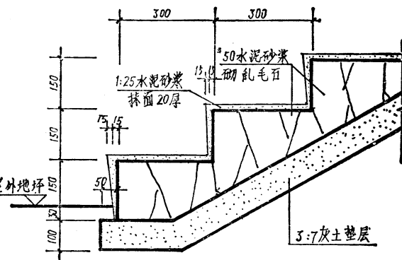
③ 乱毛石台阶
