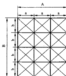
图 2 矩形风口测点布置
