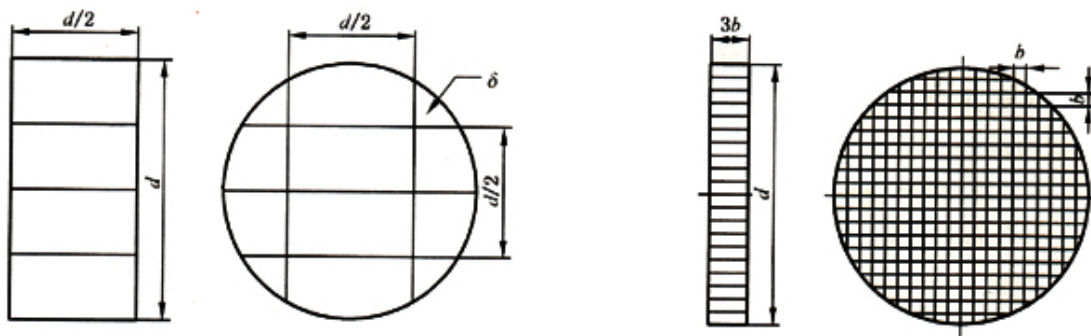
图5 进气整流栅和出气整流栅外形尺寸
