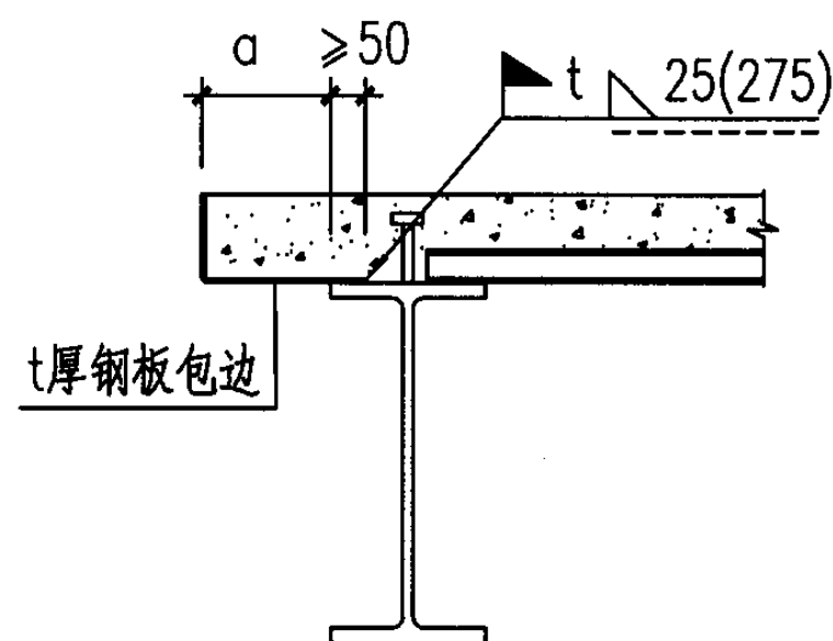
板肋与梁垂直收边构造(2) ( a \leq 250 )
