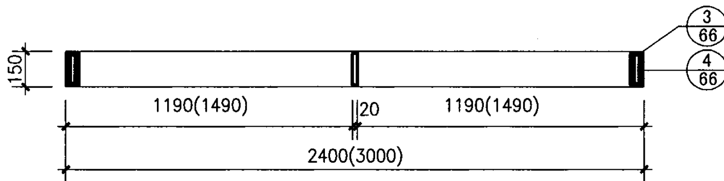
2-2 (C型)
