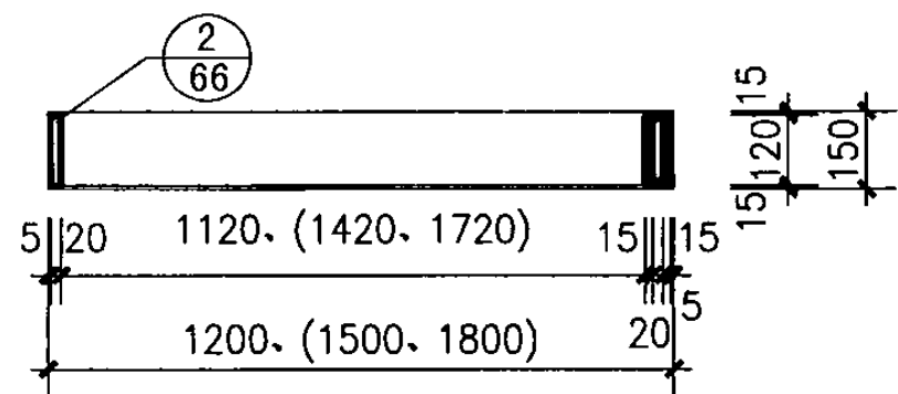
1-1 (A型)
