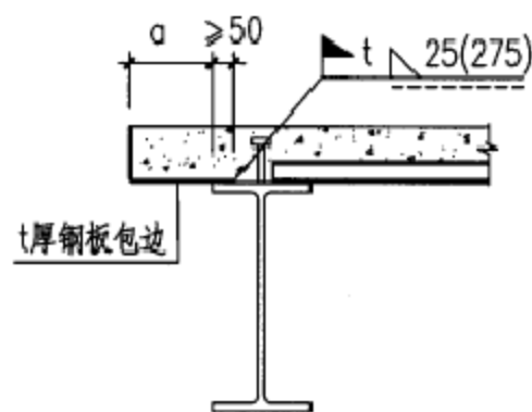
板肋与梁垂直收边构造(2) ( a \leq 250 )
