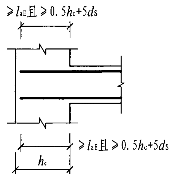
(a) 纵筋在端支座直锚
