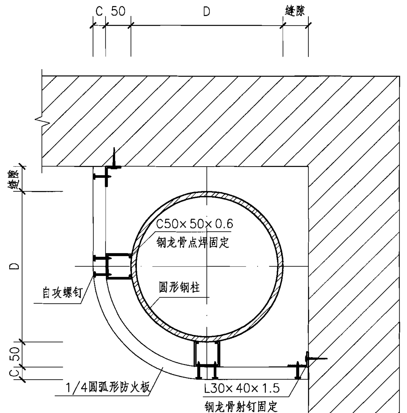
圆钢管角柱
