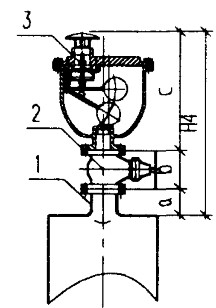
CARX复合排气阀乙型安装
